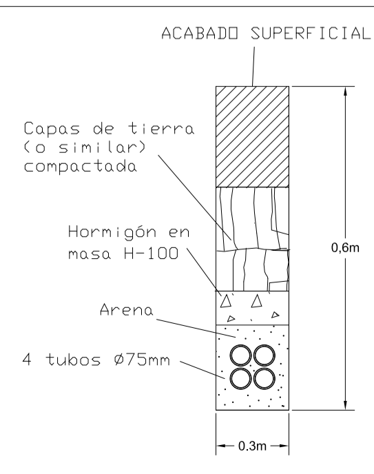
DETALL RASA CREUAMENT 4 TUBS
