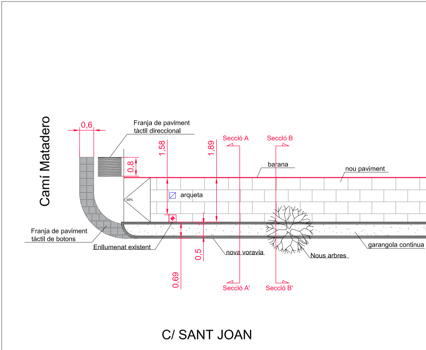
DETALL TRAM 1 (E 1/100)
